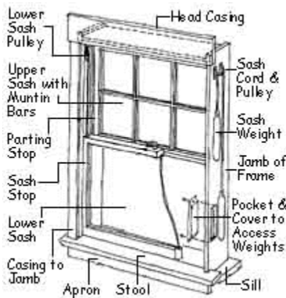
Illustration: Double-Hung Window, view from inside
