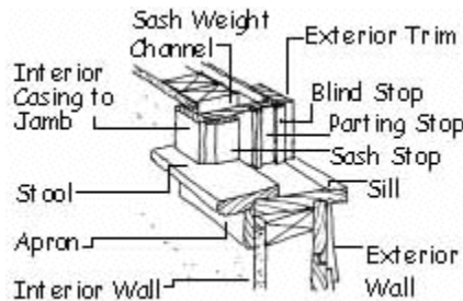
Illustration: Detail at jamb/sill junction
